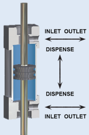
Reciprocating piston
